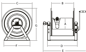
1185 SERIES MOTOR
