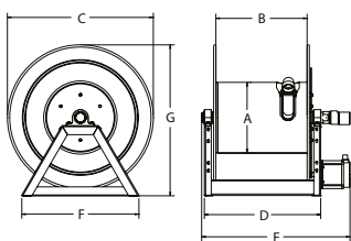
1195 SERIES MOTOR
