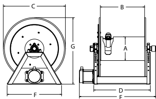
1195 SERIES MOTOR
